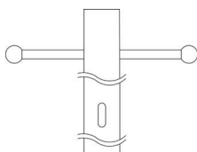
Direct Burial Aluminum Post with Ladder Rest 9501 BK, WH 3"W x 84"H
