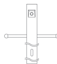
Direct Burial Aluminum Post with Ladder Rest and External Photocell 49904 AZ, BK, 3"W x 84"H
